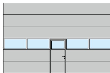
SPU F42, SPU 67 Thermo Aluminium beglazingspaneel Loopdeurpositie midden
