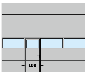
SPU F42, SPU 67 Thermo Aluminium beglazingspaneel Loopdeurpositie links
